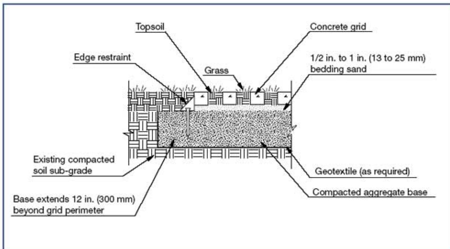
Figure 17. Typical concrete grid pavement over dense-graded base
