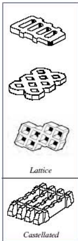
Figure 14. Types of Grid Pavement Units
