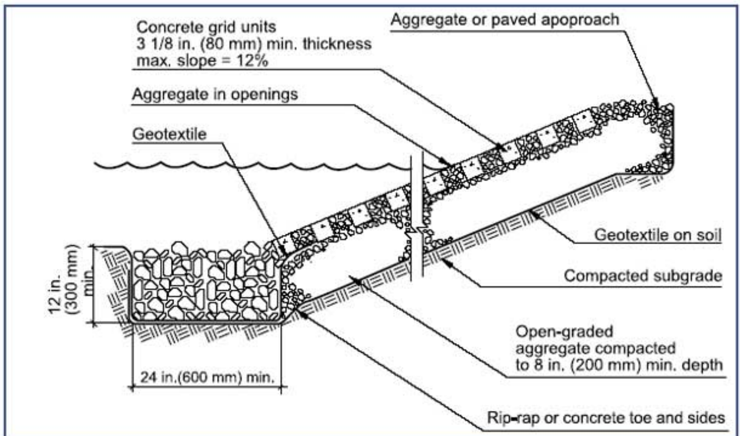
Figure 22. Typical cross-section for boat ramp
