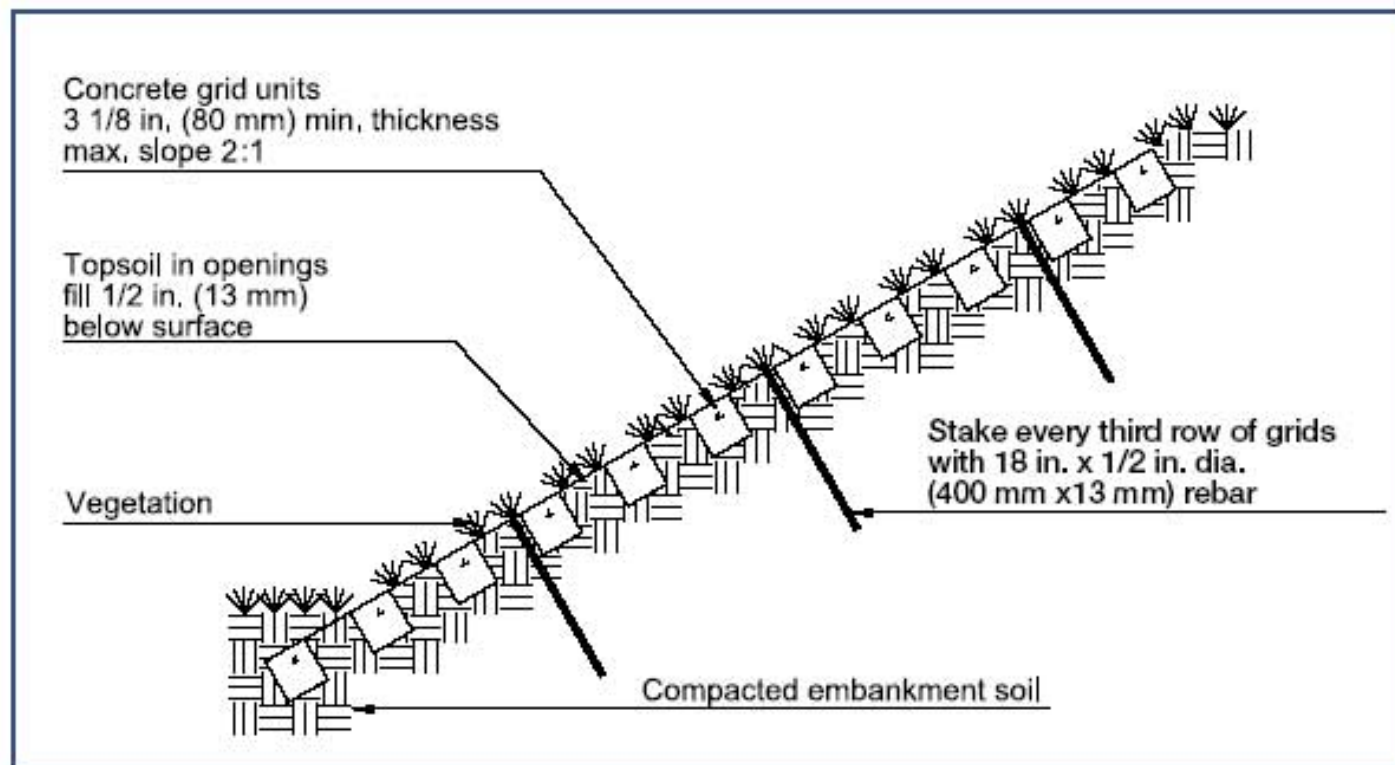
Figure 19. Embankment stabilization with concrete grids
