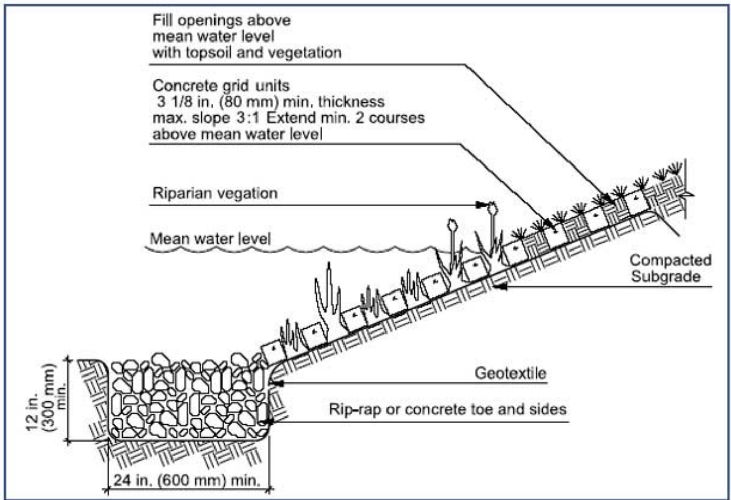
Figure 21. Lake side stabilization with concrete grids
