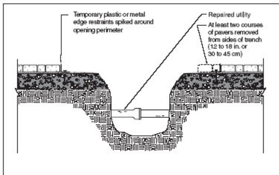
Figure 8. T-shaped cross section of the excavated opening
