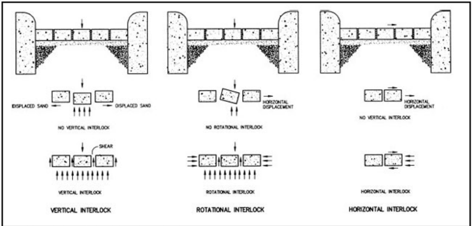
Figure 2. Types of interlock: vertical, rotational, horizontal.
