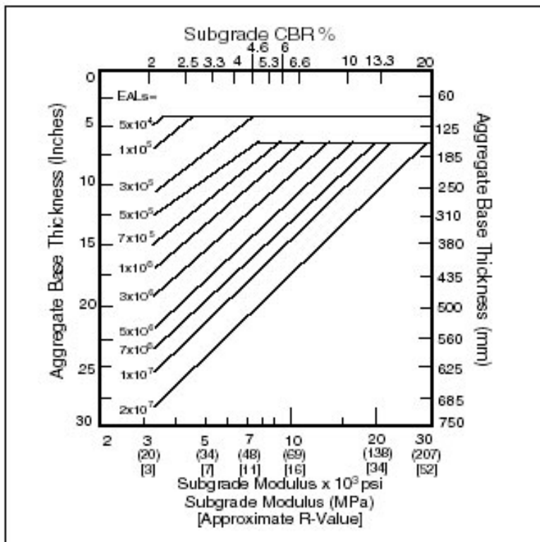
Figure 5. Thickness design curves—aggregate base.
