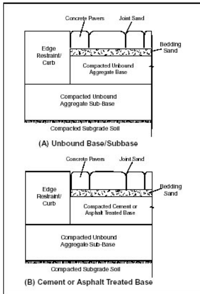
Figure 4. Typical schematic cross sections.
