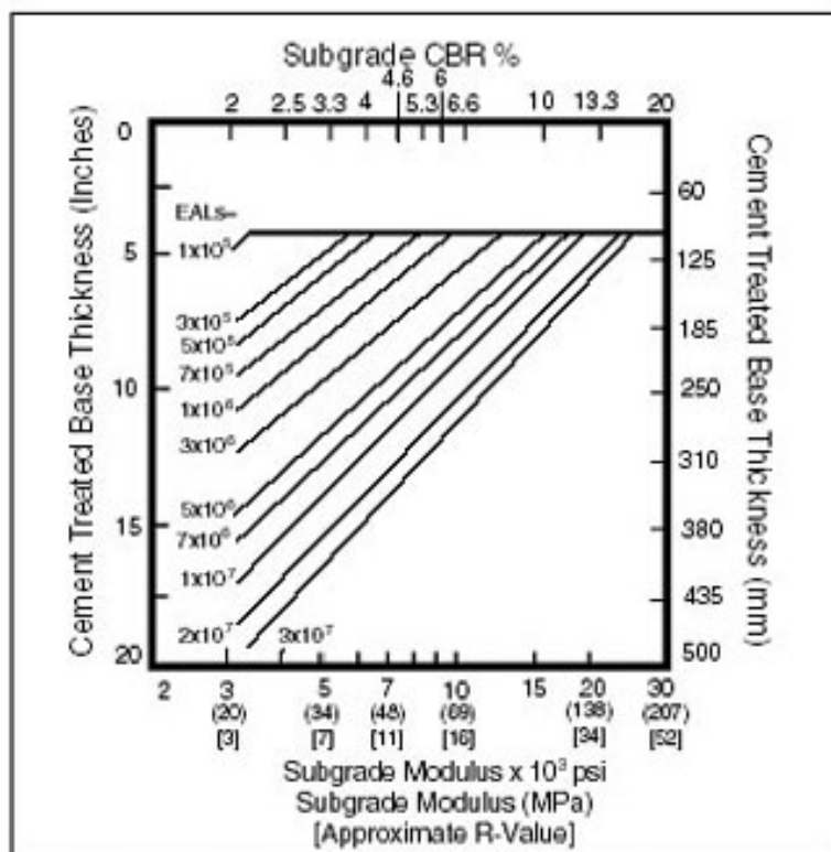
Figure 7. Thickness design curves— cement treated base.
